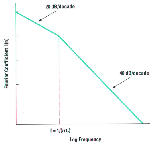
Fig. 6. The envelope of the Fourier series of a trapezoidal waveform has a breakpoint that depends purely upon the rise time ( \tau_r ). Slowing down the rise time shifts this breakpoint down in frequency and reduces the amplitude of the high-frequency harmonics.
