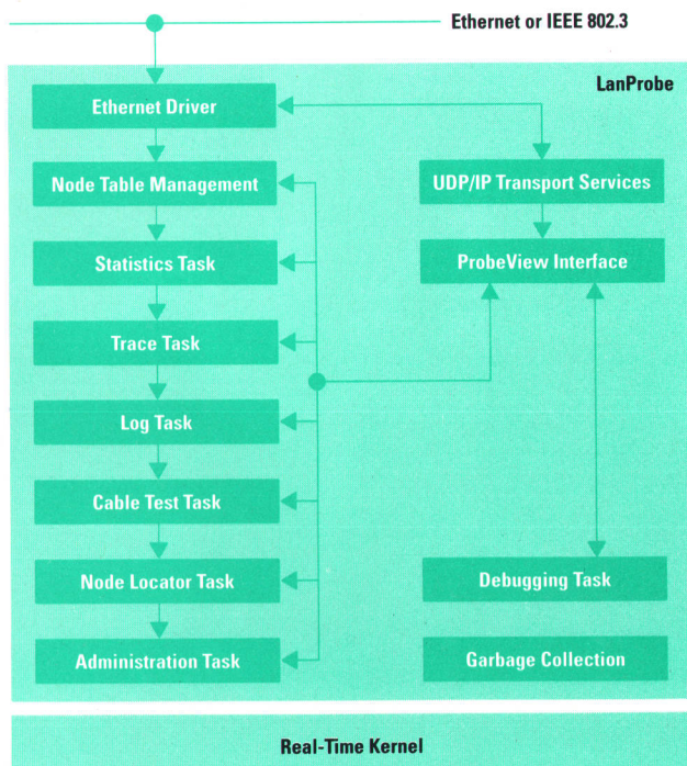
Fig. 8. HP LanProbe internals and tasks.
