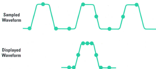
Fig. 1. Random repetitive sampling.
