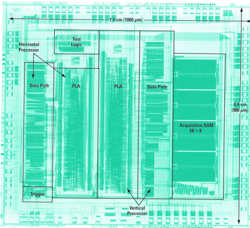
Fig. 6. Acquisition processor chip layout.
