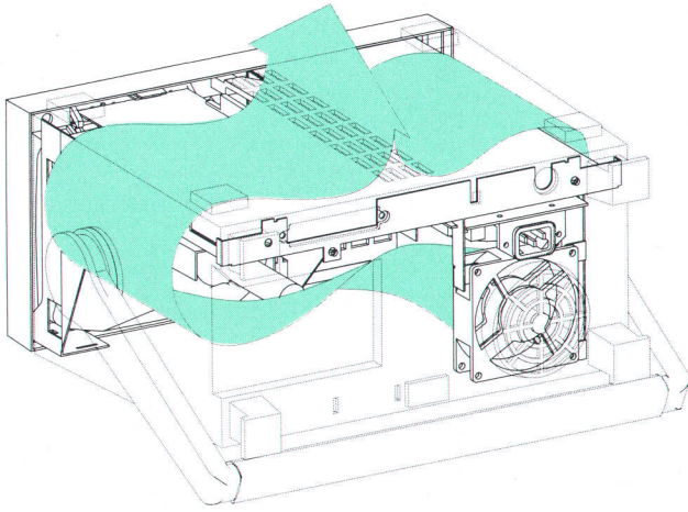
Fig. 5. Airflow in the HP 54600 Series.
