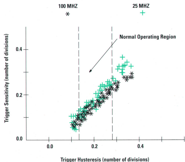
Fig. 6. Plot showing the linear relationship between hysteresis and trigger sensitivity.
