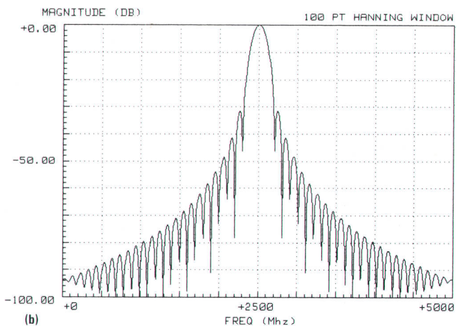
Fig. 7. Frequency spectrum for (a) a 100-point rectangular window and (b) a 100-point Hanning window.
