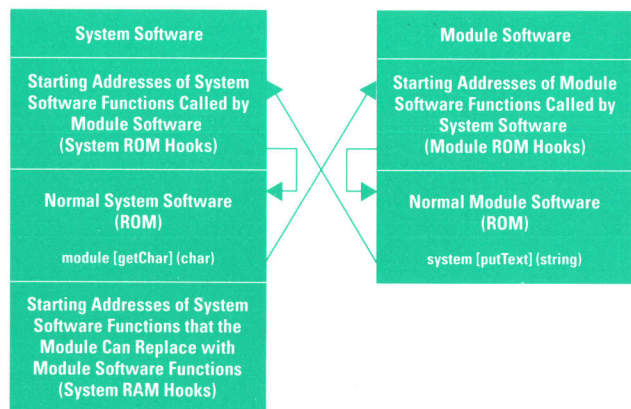
Fig. 3. RAM and ROM look-up tables contain "hooks" that are used for communication between the module software and the software of the system under test.
