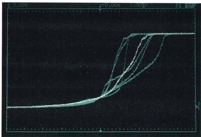
Fig. 3. Power-up characteristics of a power supply over the specified load current range, with the most recent cycle at full intensity.
