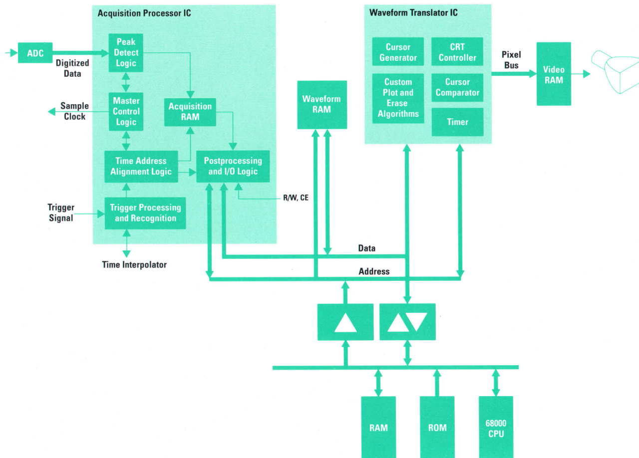
Fig. 3. New raster digital oscilloscope architecture.
