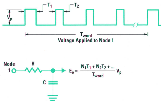
Fig. 2. Filter section input waveform and output voltage.
