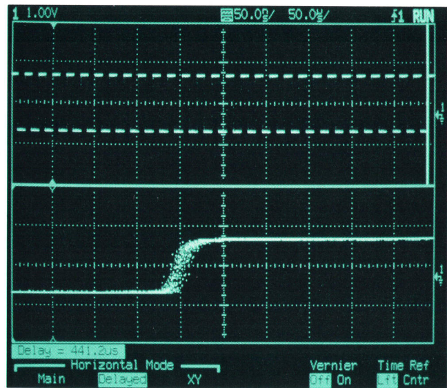
Fig. 4. HP 54600 delayed sweep display.
