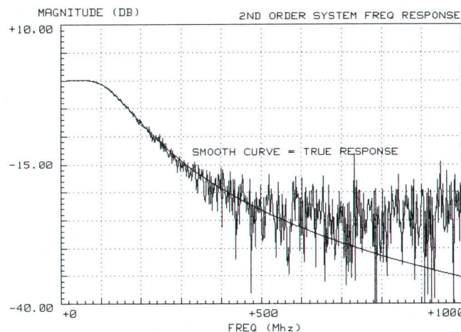
Fig. 5. True frequency response of a second-order system compared with the estimated response.
