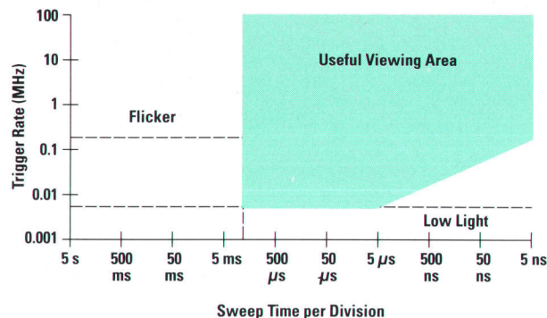
Fig. 1. Analog oscilloscope operating area.
