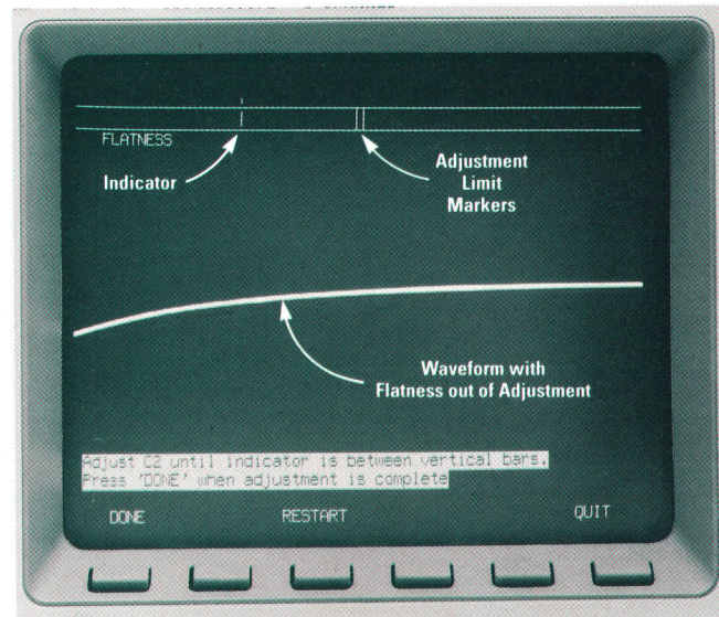
Fig. 4. Flatness adjustment display.
