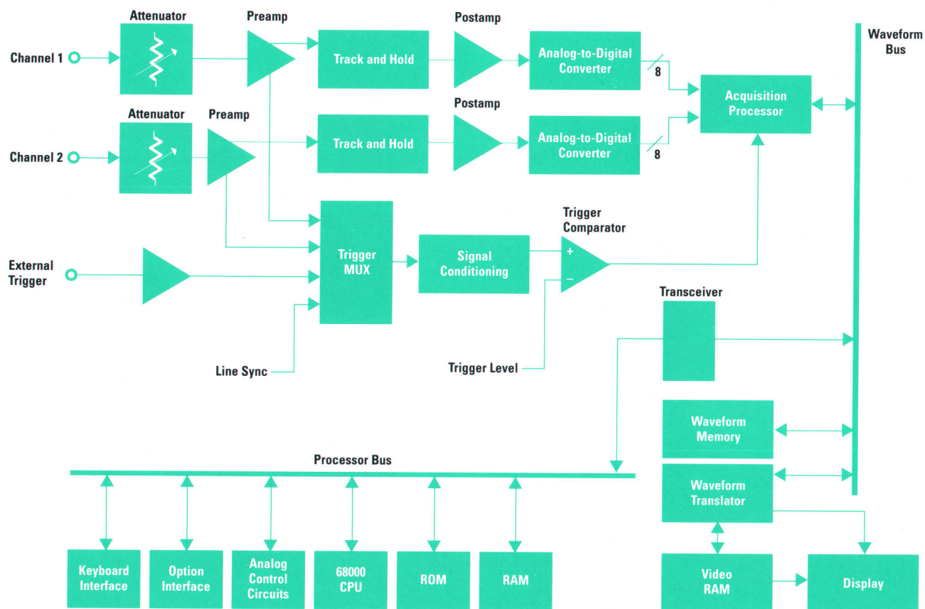
Fig. 5. Simplified block diagram of the HP 54600A two-channel oscilloscope.
